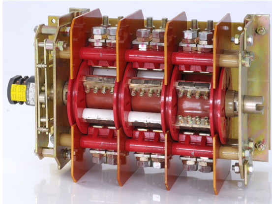
GLC79-800/3.6 AC vacuum contactor
